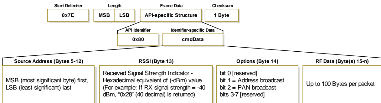
Figure 4-13. RX Packet (64-bit address) Frames
