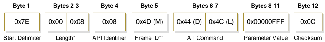
Figure 4-07. Example: API frames when modifying the DL parameter value of the modem.
