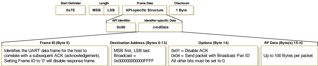
Figure 4-10. TX Packet (64-bit address) Frames
