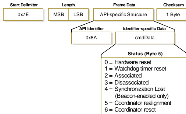
Figure 4-04. Modem Status Frames
