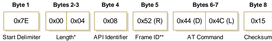
Figure 4-06. Example: API frames when reading the DL parameter value of the modem.
