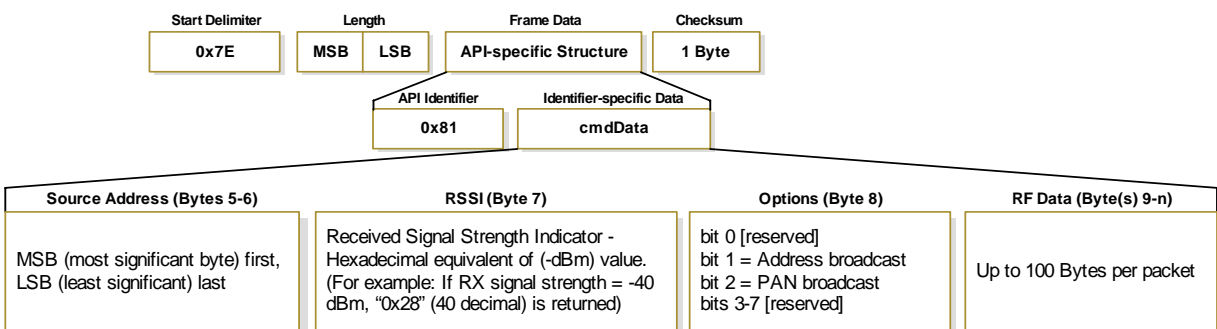
Figure 4-14. RX Packet (16-bit address) Frames
