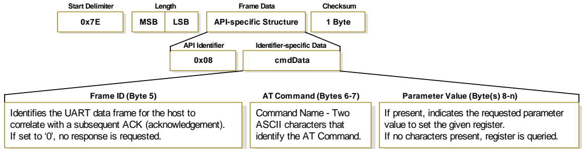
Figure 4-06. Example: API frames when reading the DL parameter value of the modem.
