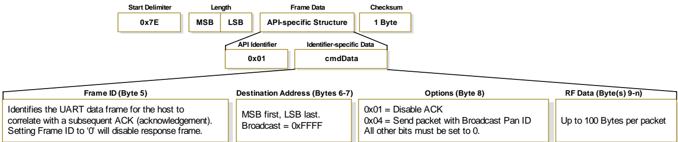
Figure 4-11. TX Packet (16-bit address) Frames
