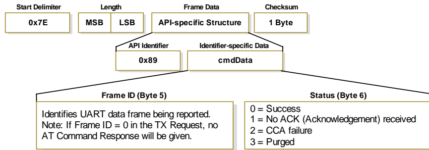
Figure 4-12. TX Status Frames
