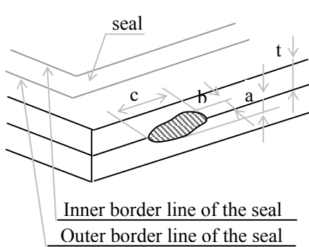
③ Surrounding crack— contact side
