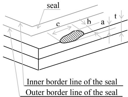
②Surrounding crack—non-contact side seal
